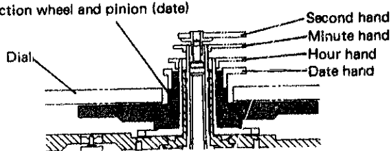
Installing the hour and minute hands
