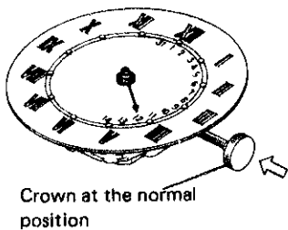
Installing the date hand
